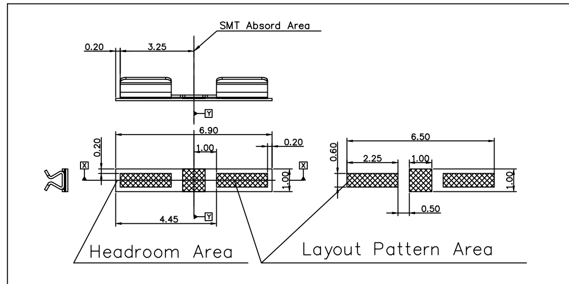
PCB Recommend Layout Pattern
