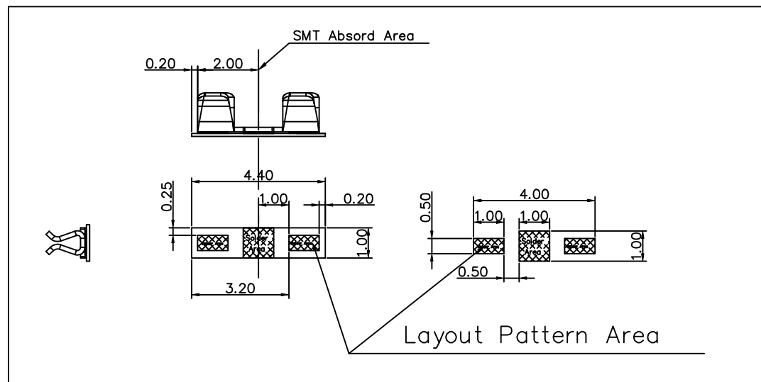
PCB Recommend Layout Pattern
