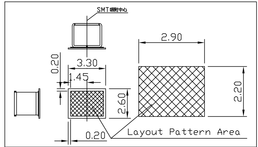
PCB Recommend Layout Pattern
