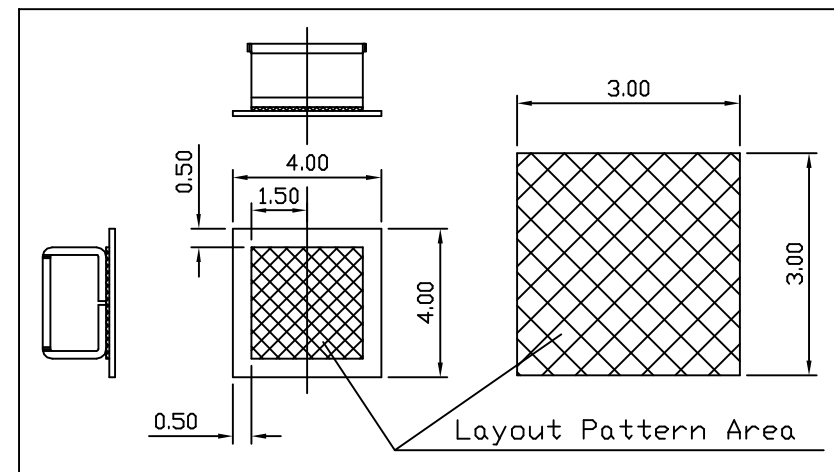
PCB Recommend Layout Pattern
